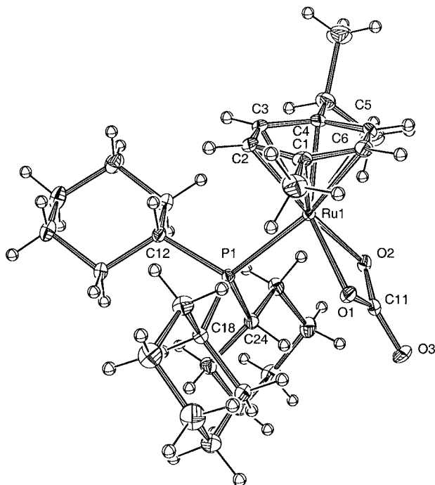
Figure 1. ORTEP drawing of 2a ·1/2 \text{CH}_2\text{Cl}_2 showing 50% probability thermal ellipsoids. The \text{CH}_2\text{Cl}_2 molecule has been omitted for clarity. Selected bond lengths [Å] and angles [°]: Ru1–O1 2.079(2), Ru1–O2 2.087(2), O1–C11 1.323(3), O2–C11 1.315(3), O3–C11 1.232(3), Ru1–P1 2.3779(6); O1–Ru1–O2 62.90(7), C11–O1–Ru1 93.02(1), C11–O2–Ru1 92.90(1), O1–C11–O2 111.0(2), O1–C11–O3 124.5(2), O2–C11–O3 124.5(2), O1–Ru1–P1 86.92(5), O2–Ru1–P1 88.09(5).
