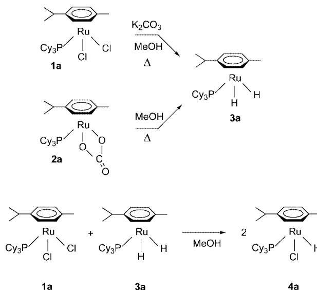
Scheme 2. Synthesis of the ruthenium hydride complexes 3a and 4a .
