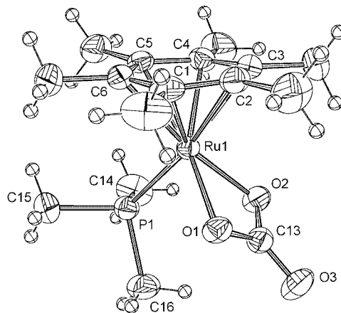
Figure 2. ORTEP drawing of 2d · \text{H}_2\text{O} showing 50% probability thermal ellipsoids. The \text{H}_2\text{O} molecule has been omitted for clarity. Selected bond lengths [Å] and angles [°]: Ru1–O1 2.104(2), Ru1–O2 2.091(2), O1–C13 1.325(4), O2–C13 1.315(4), O3–C13 1.239(4), Ru1–P1 2.343(1); O1–Ru1–O2 62.81(8), C13–O1–Ru1 92.2(2), C13–O2–Ru1 93.1(2), O1–C13–O2 111.8(2), O1–C13–O3 123.7(3), O2–C13–O3 124.5(3), O1–Ru1–P1 88.61(7), O2–Ru1–P1 84.25(7).
