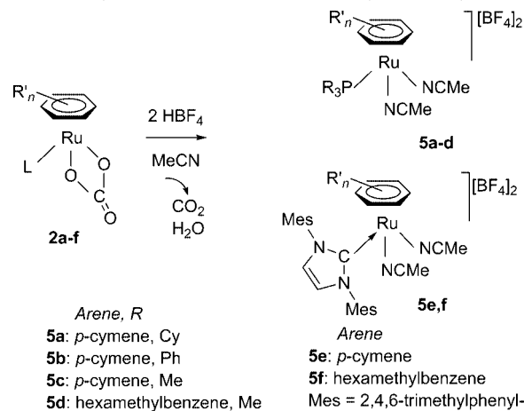
Scheme 5. Synthesis of the dicationic derivatives [\text{Ru}(\eta^6\text{-arene})(\text{L})(\text{MeCN})_2][\text{BF}_4]_2 ( 5a–f ).
