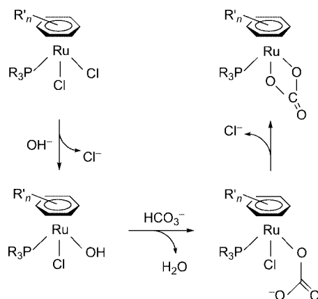
Scheme 3. Rationale accounting for the formation of complexes 2 catalysed by water.
