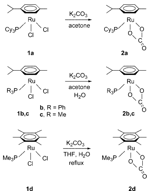
Scheme 1. Synthesis of the new carbonatoruthenium complexes 2a–d .
