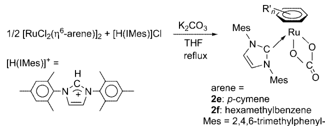
Scheme 4. Synthesis of the carbonatoruthenium complexes [\text{Ru}(\eta^2\text{-O}_2\text{CO})(\eta^6\text{-arene})(\text{IMes})] ( 2e and 2f ).
